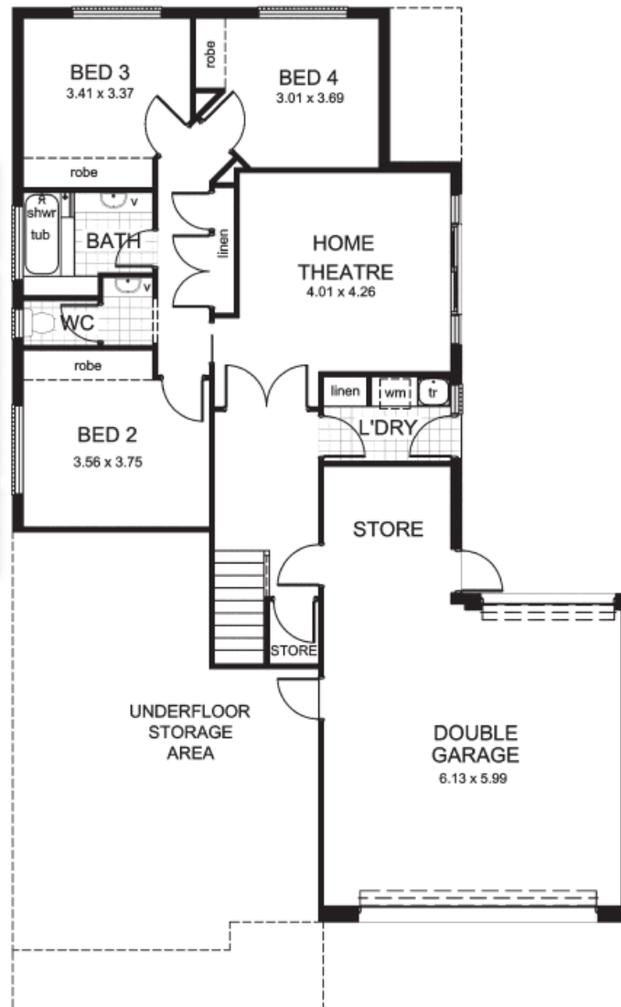
LOWER LEVEL
