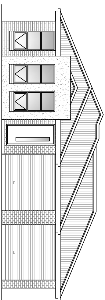
ELEVATION (FRONT) SCALE: 1:100
